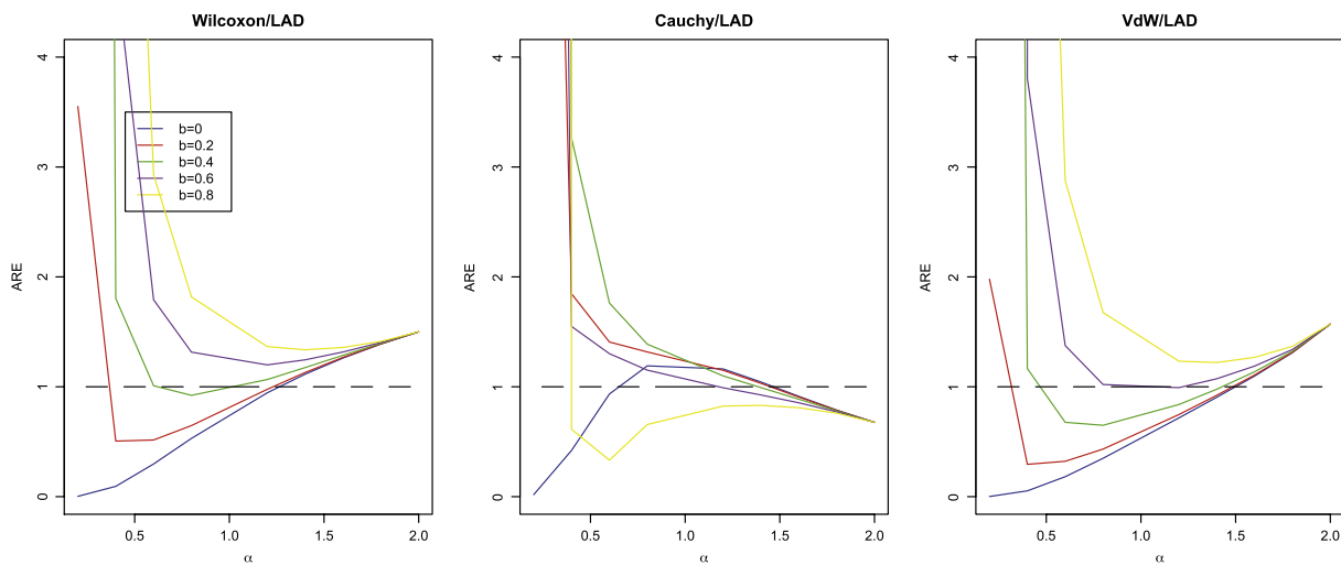
Fig. 1. AREs of R-estimators based on Wilcoxon, Cauchy and van der Waerden scores, with respect to the LAD estimator, as a function of \alpha and for various values of b .
