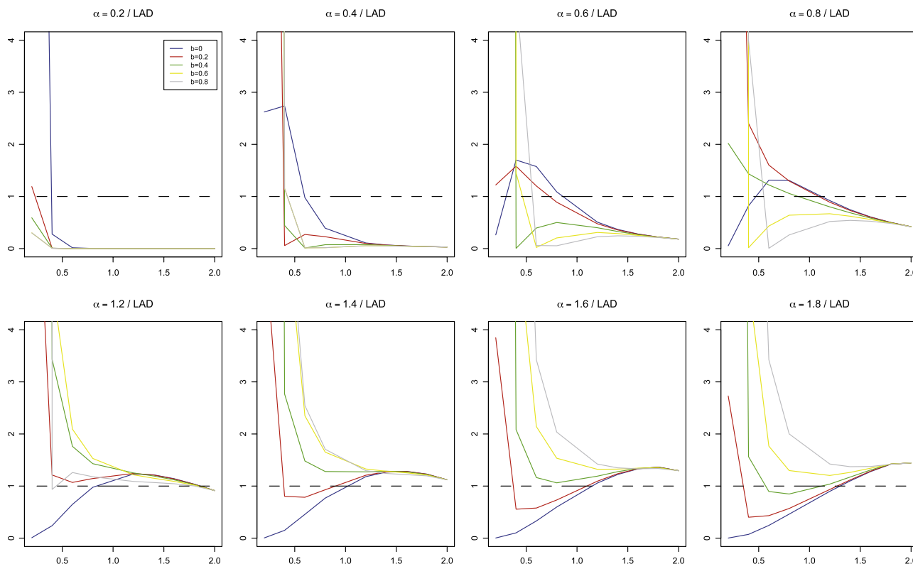
Fig. 2. AREs under stable distributions of R-estimators based on various stable scores with respect to the LAD estimator, as a functions of \alpha and b .
